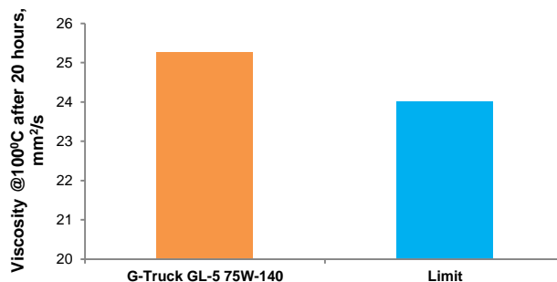
Shear Stability**
