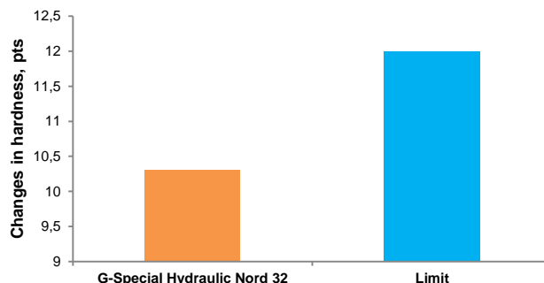
Elastomer Compatibility**
